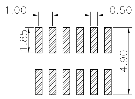
RECOMMENDED PCB LAYOUT (COMPONENT SIDE) (TOLERANCE: ±0.05)
